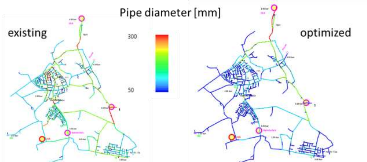
Figure 3: Result of diameter optimization using Linear Programming
